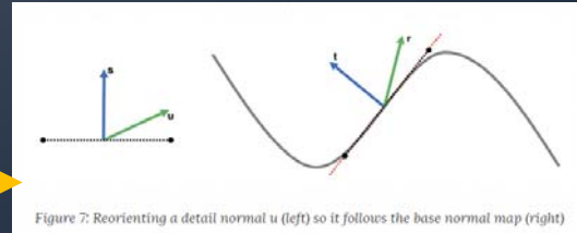
Figure 7: Reorienting a detail normal u (left) so it follows the base normal map (right)
